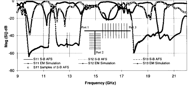
Fig. 10. Magnitude of S -parameters of a microstrip broad-band diplexer obtained by the S-B AFS and direct EM simulation with 1001 sampling points of equal space.
