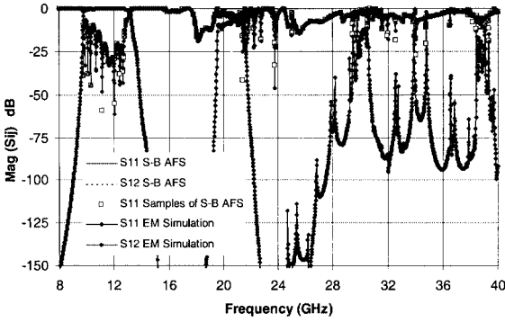
Fig. 8. S -parameters of hidden spurious harmonic modes of a low-pass corrugated waveguide filter calculated by the S-B AFS and full-wave EM simulation with 2001 samples.
