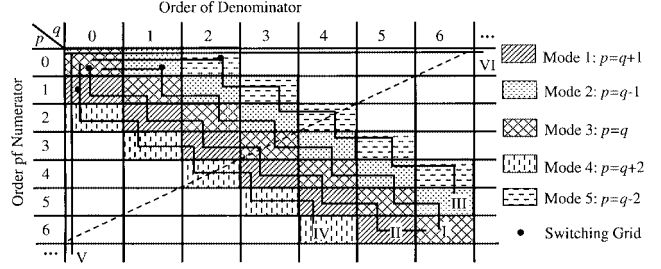
Fig. 1. Grid paths of possible rational functions of FMs.
