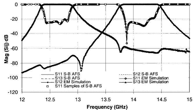
Fig. 6. Magnitude of S -parameters of a waveguide diplexer calculated by the S-B AFS and full-wave EM simulation with 501 samples.
