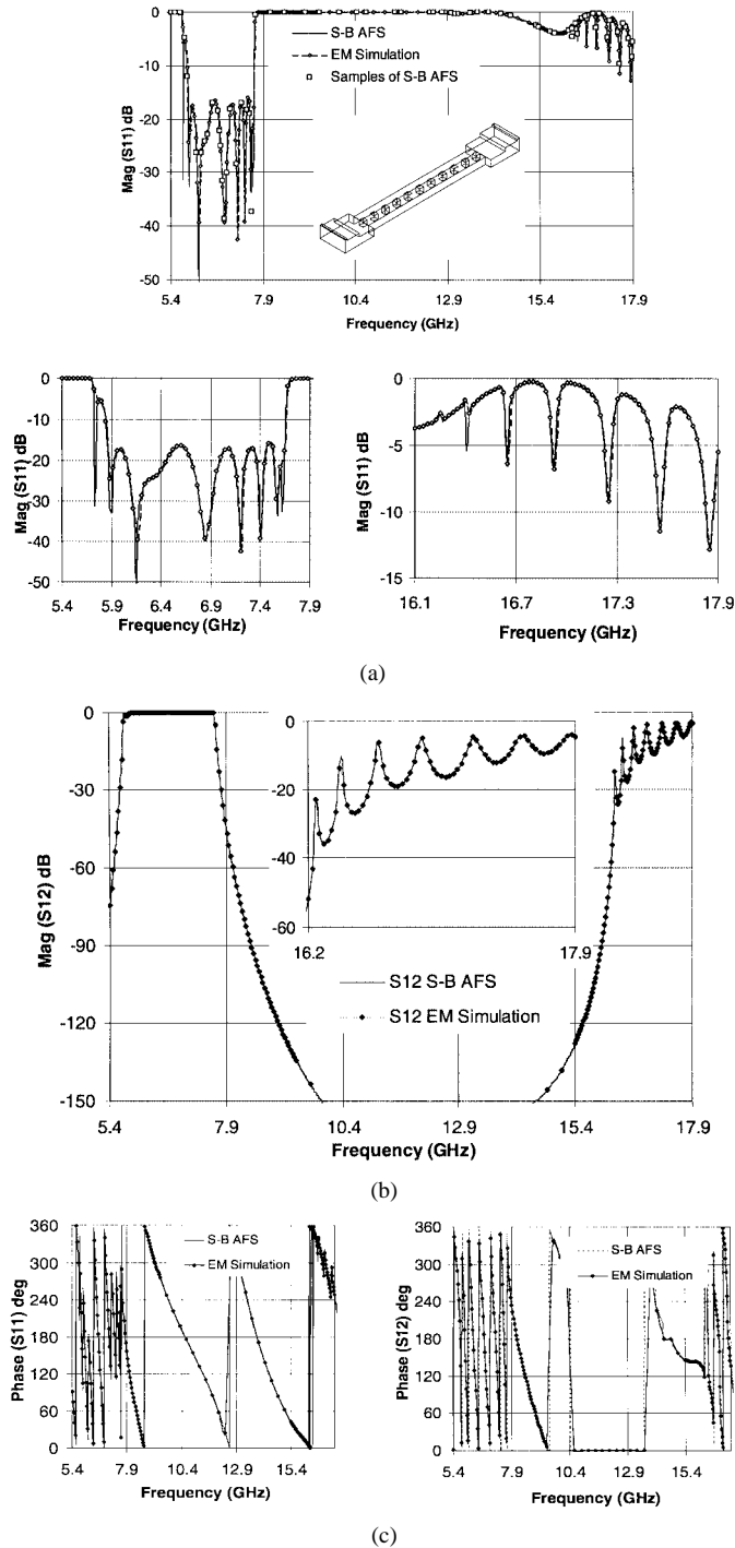
Fig. 3. (a) Magnitude of S_{11} of an 11-pole waveguide filter calculated by S-B AFS and full-wave EM simulation with 501 samples. (b) Magnitude of S_{12} of an 11-pole waveguide filter calculated by S-B AFS and full-wave EM simulation with 501 samples. (c) Phase of an 11-pole waveguide filter calculated by S-B AFS and full-wave EM simulation with 501 samples.
