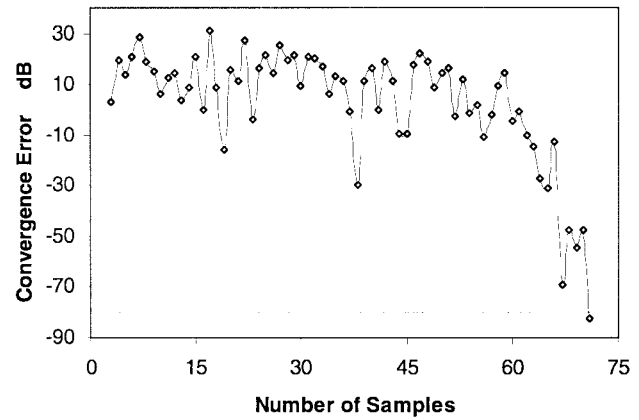
Fig. 4. Convergence error of the S-B AFS for an 11-pole waveguide filter.
