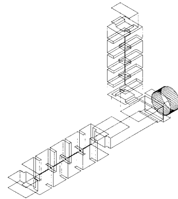
Fig. 5. Waveguide diplexer with two five-pole bandpass filters at Tx and Rx channels and a rectangular-to-circular waveguide transition at the common port.
