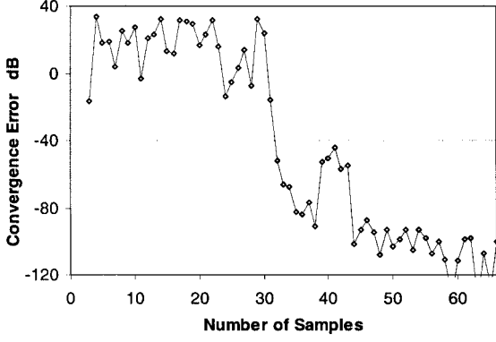
Fig. 7. Convergence error of the S-B AFS for the waveguide diplexer.
