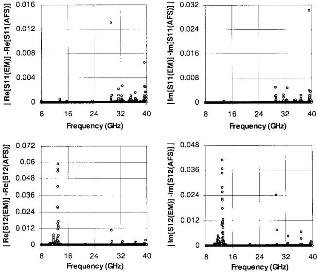
Fig. 9. Error of the FMs of the low-pass corrugated waveguide filter.
